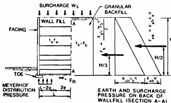
Figure 3 External Design Forces
