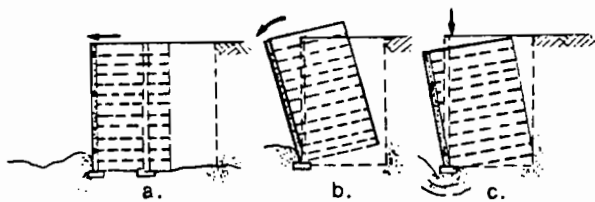
Figure 2 Modes of Wall Failure: a) sliding, b) over- turning, and c) bearing.
