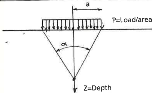
Figure 3. Variables for the calculation of vertical stress in subgrade.
