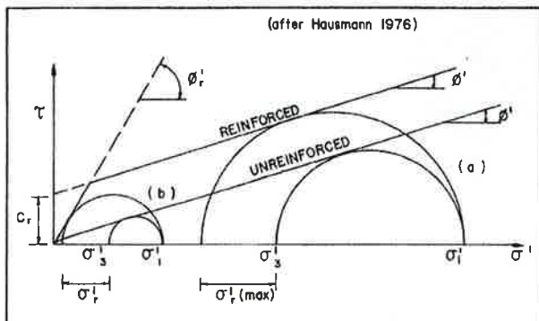
Figure 1. Composite Mohr envelope; reinforced earth.
